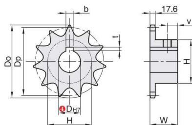
链轮 CD21GF
