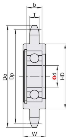
单轴承 CD23AF/CD23AU
