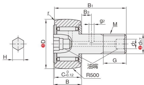
圆弧型•不带密封圈型 CA76CS/CA76CH
