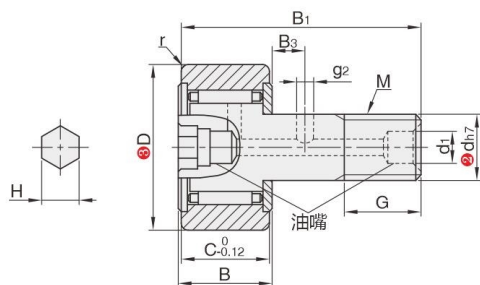
圆柱型•不带密封圈型 CA76AS/CA76AH
