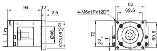
电机连接法兰MKK100-F4 (86步进电机)
