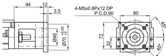
电机连接法兰MKK100-F4 (86步进电机)
