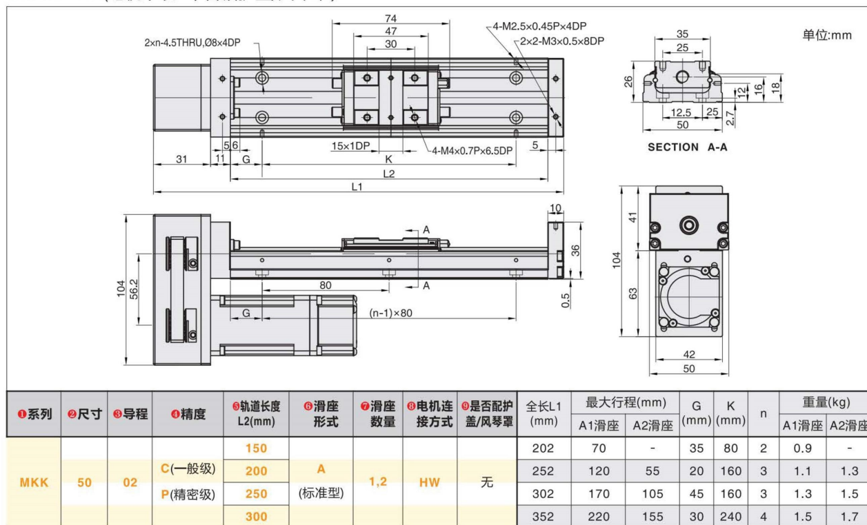
MKK50-HW (电机下装+不含铝护盖/风琴罩)
