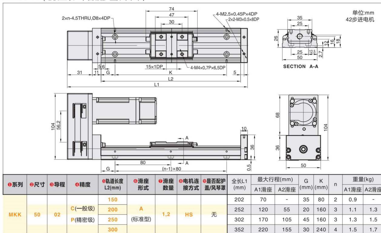
MKK50-HS (电机上装+不含铝护盖/风琴罩)
