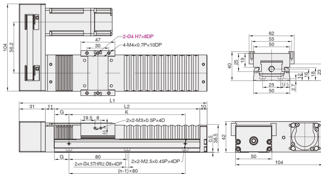
MKK50-HRB (电机右装+风琴罩)
