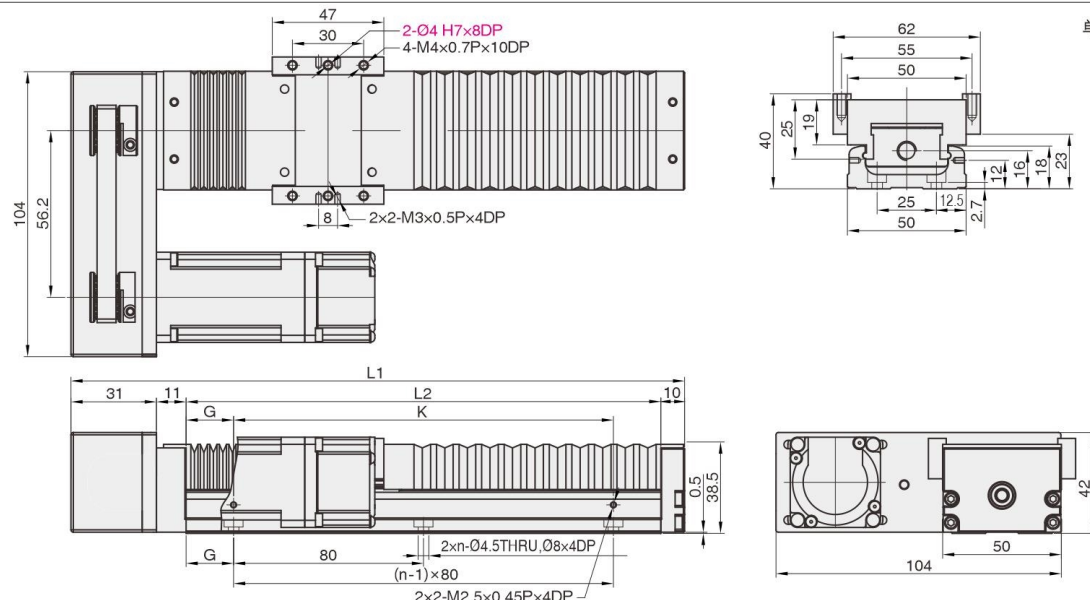
MKK50-HLB (电机左装+风琴罩)
