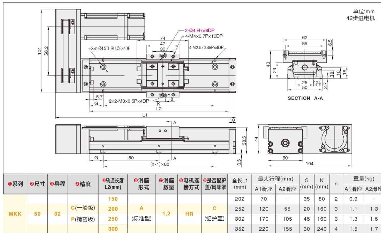
MKK50-HRC (电机右装+铝护盖)
