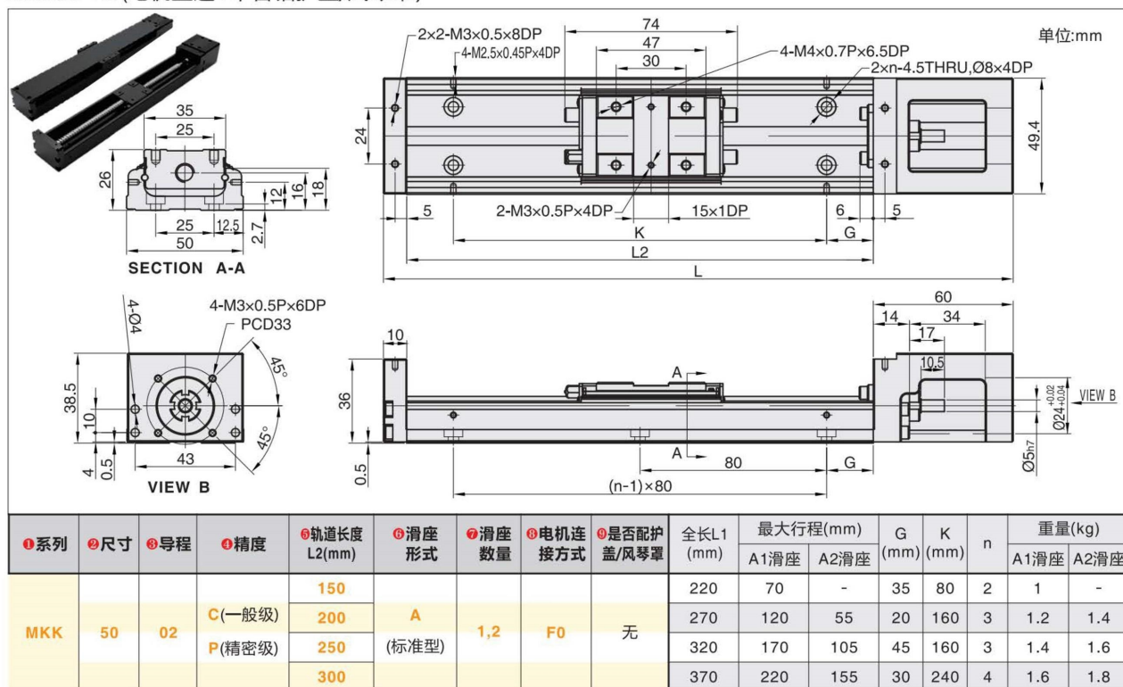
MKK50-F0 (电机直连+不含铝护盖/风琴罩)
