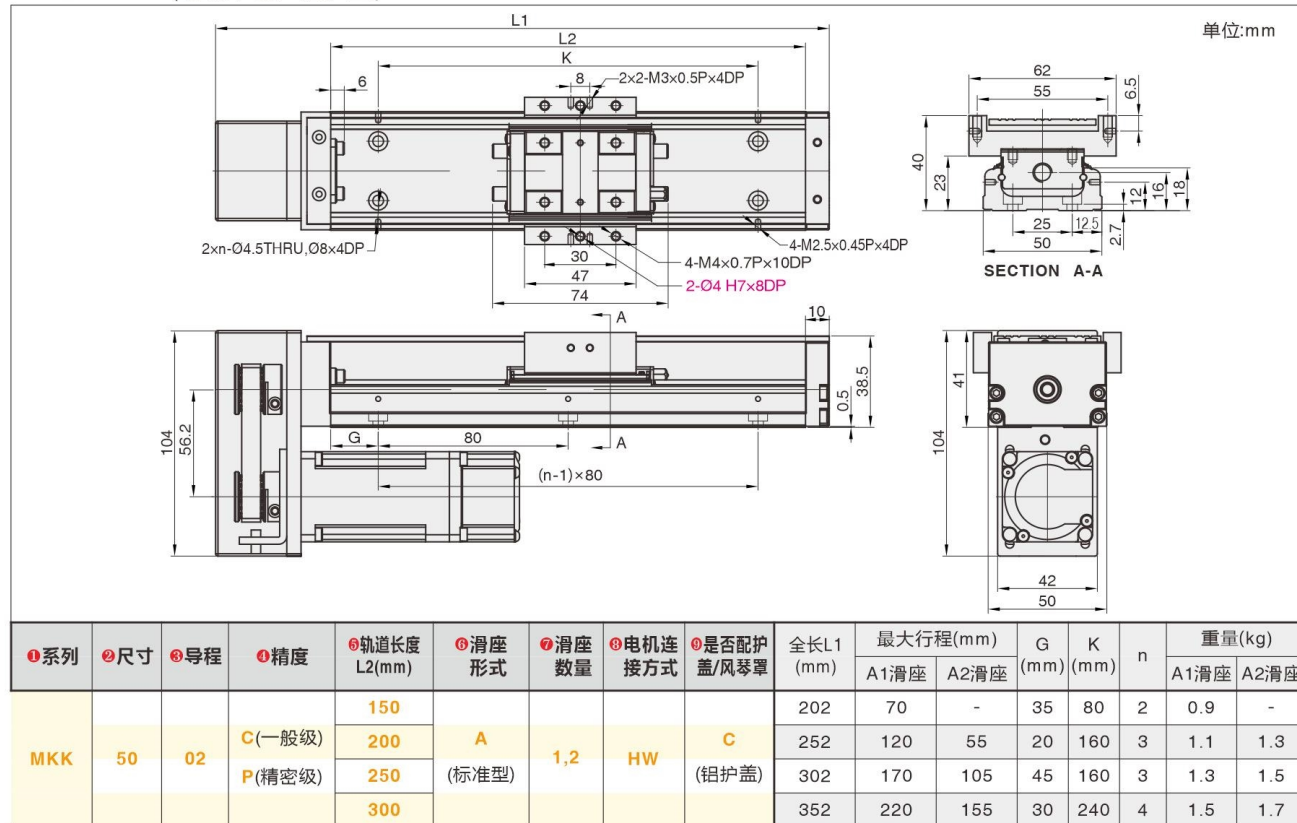
MKK50-HWC (电机下装+铝护盖)
