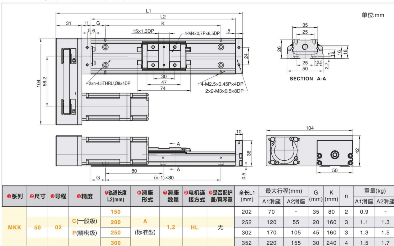
MKK50-HL (电机左装+不含铝护盖/风琴罩)
