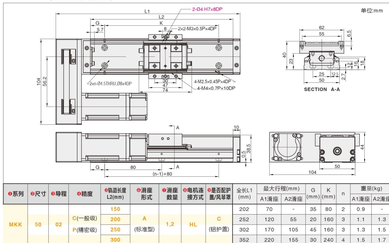
MKK50-HLC (电机左装+铝护盖)
