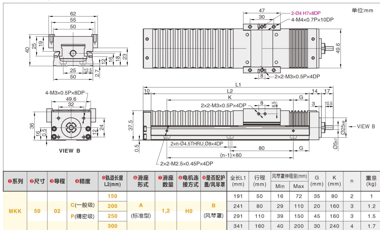
MKK50-H0B (无电机座+风琴罩)
