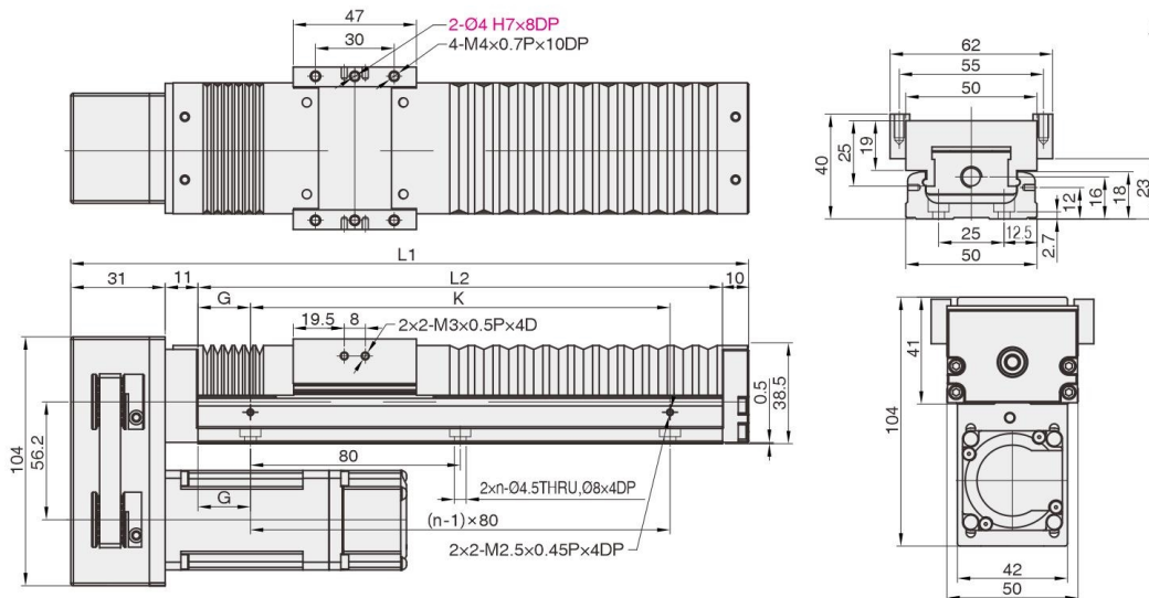
MKK50-HWC (电机下装+风琴罩)
