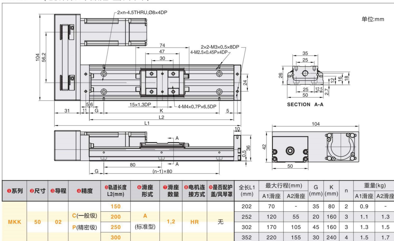
MKK50-HR (电机右装+不含铝护盖/风琴罩)
