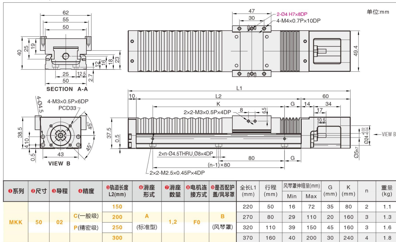
MKK50-F0B (电机直连+风琴罩)
