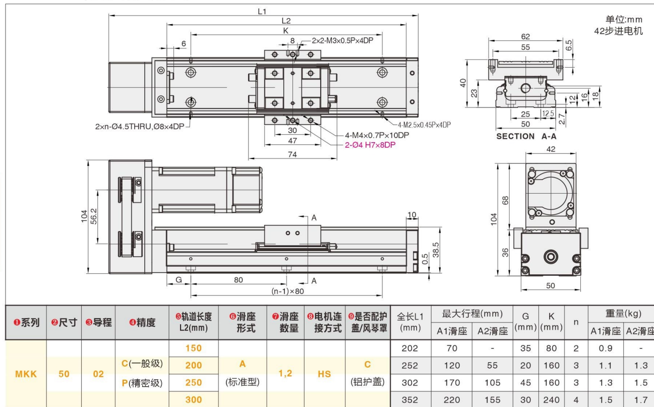
MKK50-HSC (电机上装+铝护盖)
